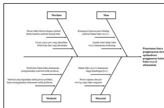
Gambar 3. Diagram Fishbone
